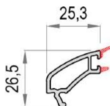
BW 3041 4mm PVC LAJSNA SLIDING GLAZING BEAD
