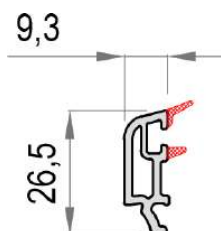
BW 7054 20mm PVC LAJSNA SLIDING GLAZING BEAD
