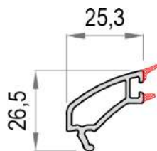
BW 7054 20mm PVC LAJSNA SLIDING GLAZING BEAD
