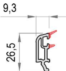
BW 7054 20mm PVC LAJSNA SLIDING GLAZING BEAD
