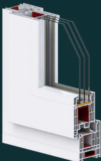
THREE-LAYERED GLASS TROSLOJNO STAKLO
