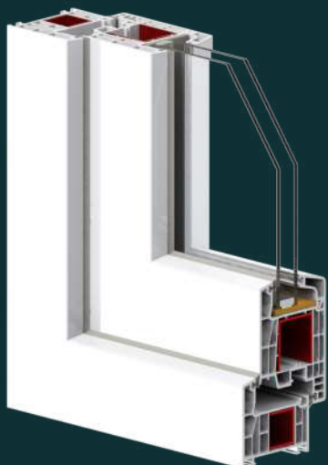
TWO-LAYERED GLASS DVOSLOJNO STAKLO
