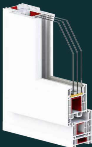
THREE-LAYERED GLASS TROSLOJNO STAKLO
