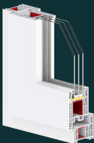
THREE-LAYERED GLASS TROSLOJNO STAKLO
